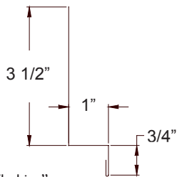
"Sidewall Flashing"
