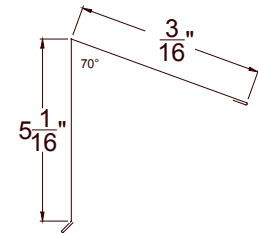
"Monoslope Ridge Flashing"
