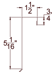
"Gable Flashing"
