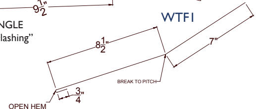
"Transition Flashing"
