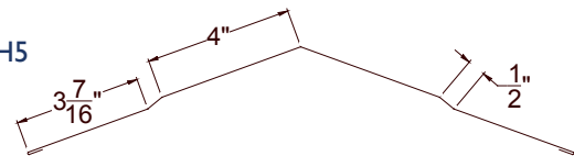
"Standard Ridge Flashings"
