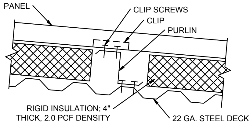
RIGID INSULATION OVER METAL DECK WITH PURLINS
