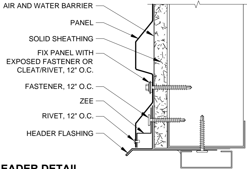
HEADER DETAIL
